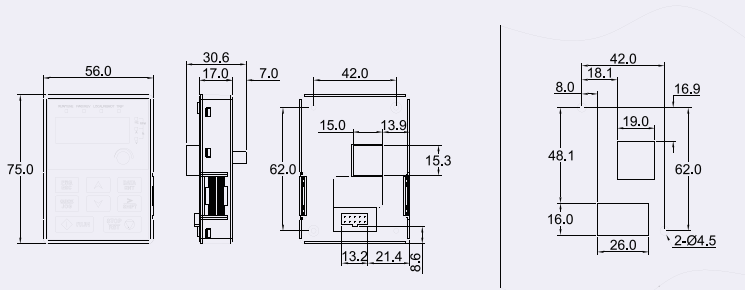
Overall drawing
